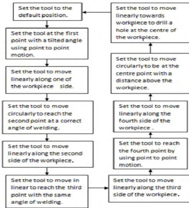
operation flow of the developed welding process.
